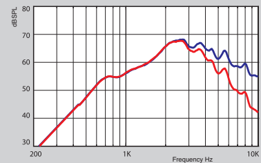
BLUE CURVE = Broadband white noise RED CURVE = Broadband pink noise
